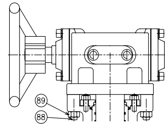
Gearbox Operator
