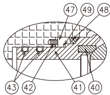
DETAIL 'A' Seat Sealing Arrangement
