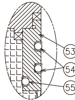
DETAIL 'B' Stem Seal Arrangement
